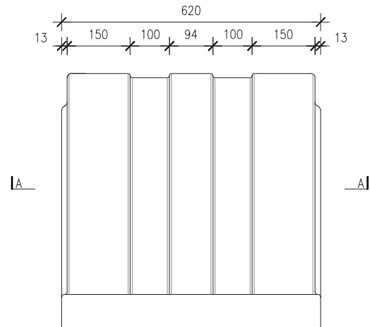
END ELEVATION (all dimensions in mm)
